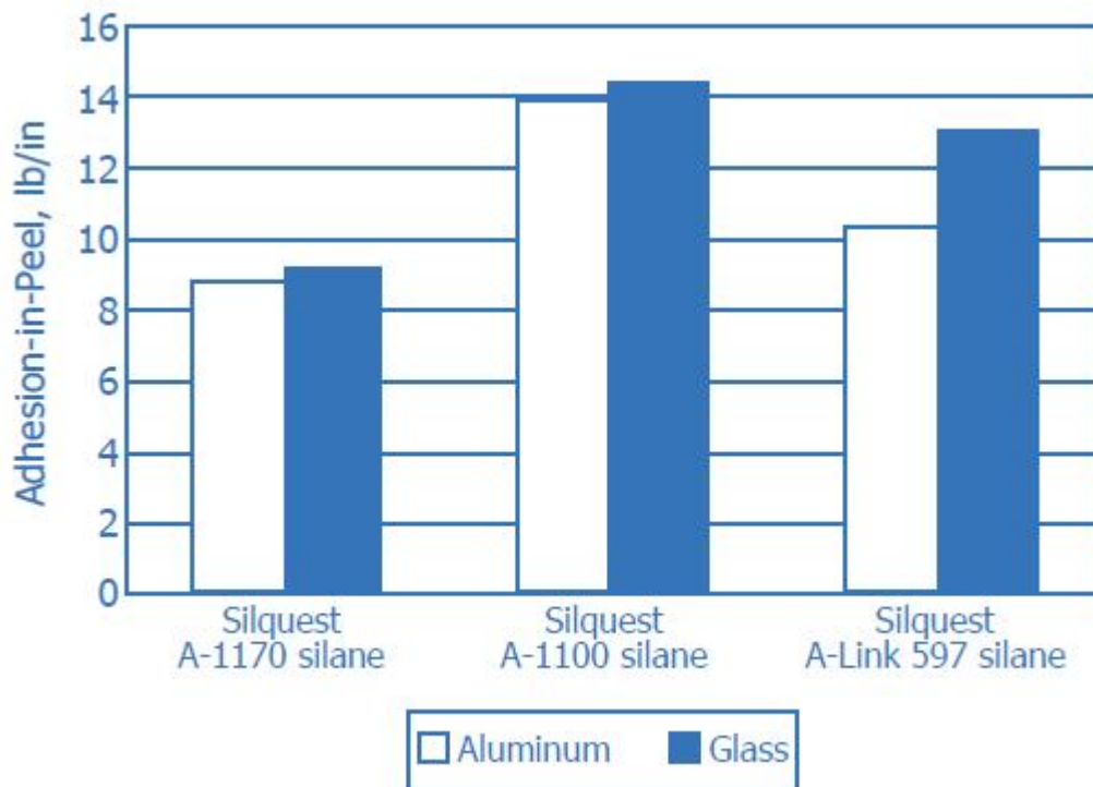
Figure 1: Adhesion-in-Peel Test
