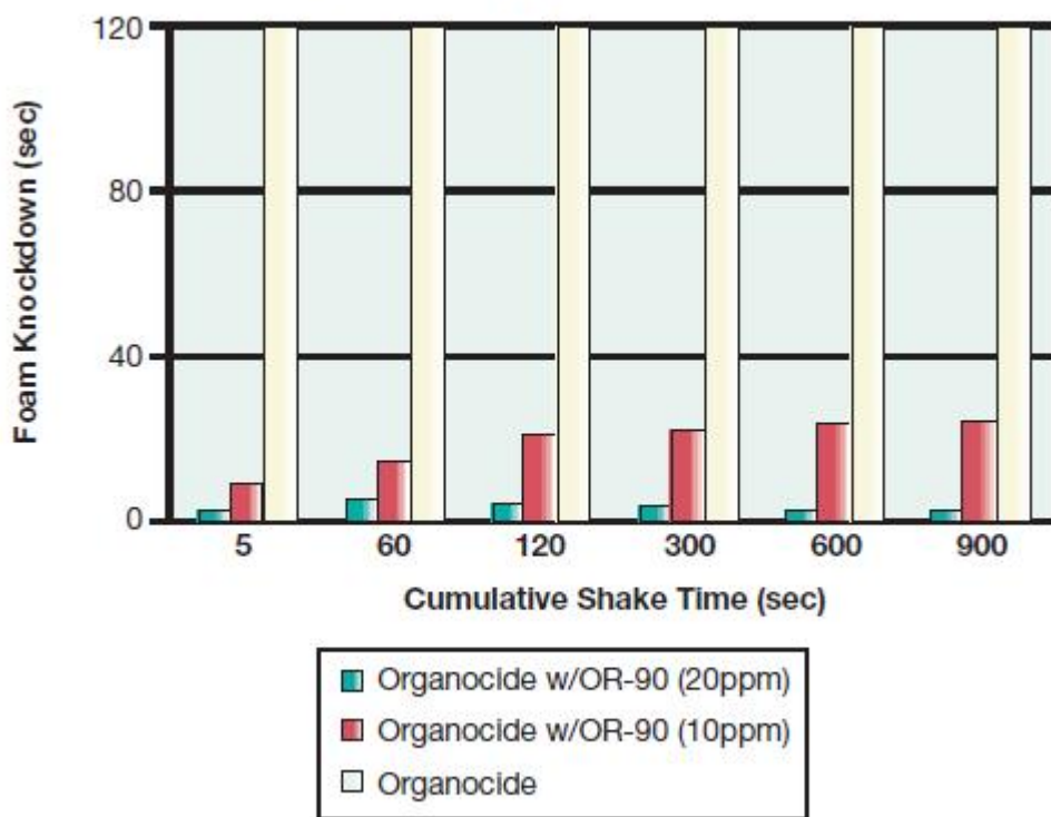
Foam control of Organocide™ (1.5%) with Antifoam OR-90
