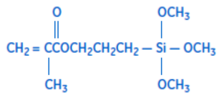
Gamma -Methacryloxypropyltrimethoxy Silane
